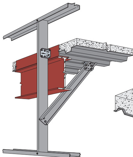
Typical FCB Installation at Sprandrel Studs and Kickers
