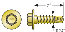
#14 Shouldered Screw
