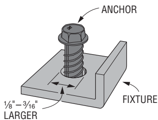
AISC 'oversized' fixture hole REQUIRED for Titen HD
