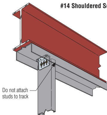
Typical SCW Installation at Stud
