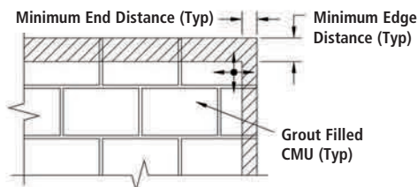
FACE SHELL Permissible Anchor Locations Un-hatched Area / Through Face Shell
