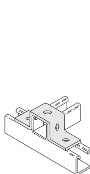
5517 5-Hole "U" Support
