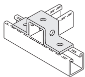
"U" SUPPORT 5501 3-Hole - 13/16" tall 5503 5-Hole - 1 5/8" tall (Shown) 5505 3-Hole - 2 7/16" tall 5507 3-Hole - 3 1/4" tall
