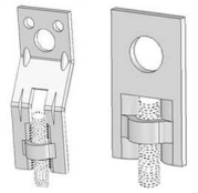
Fig. 37 Steel Eye Socket
