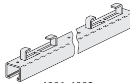
4001-4002 1 5 / 8 " X 1 3 / 8 " X 12 Gauge (Shown)
