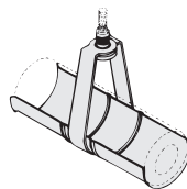
Fig. 155 Ring Hanger With Shield
