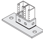
6045 Post Base for Double 1 5 / 8 Struts
