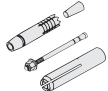
Fig. 47 Concrete Anchors
