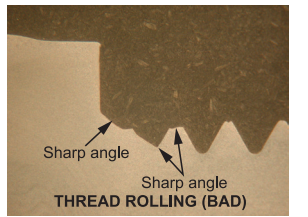
SHARP ANGLE SHARP ANGLE THREAD ROLLING (BAD)
