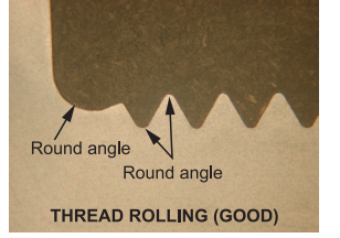
ROUND ANGLE ROUND ANGLE THREAD ROLLING (GOOD)
