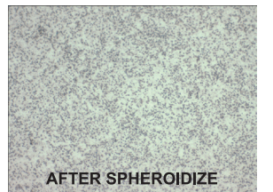
AFTER SPHEROIDIZE
